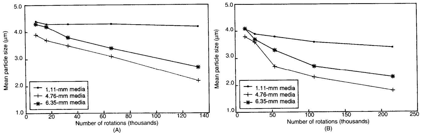
Fig. 5. Dependence of mean particle size on number of mill rotations when using zirconia media of different size: (A) 550 and (B) 900 rpm.
