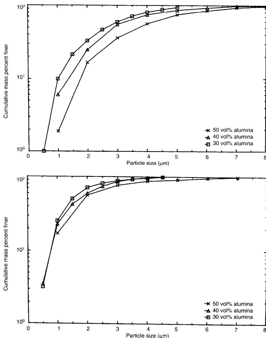
Fig. 2. Dependence of size distribution on powder loading in alumina slurry after milling for 4 h: (A) 200 and (B) 900 rpm.
