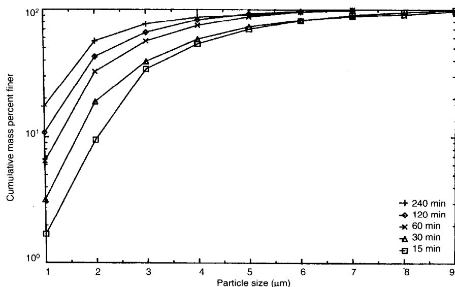
Fig. 1. Particle-size distributions for the 50 vol% alumina slurries milled using 4.76-mm zirconia media at 900 rpm.
