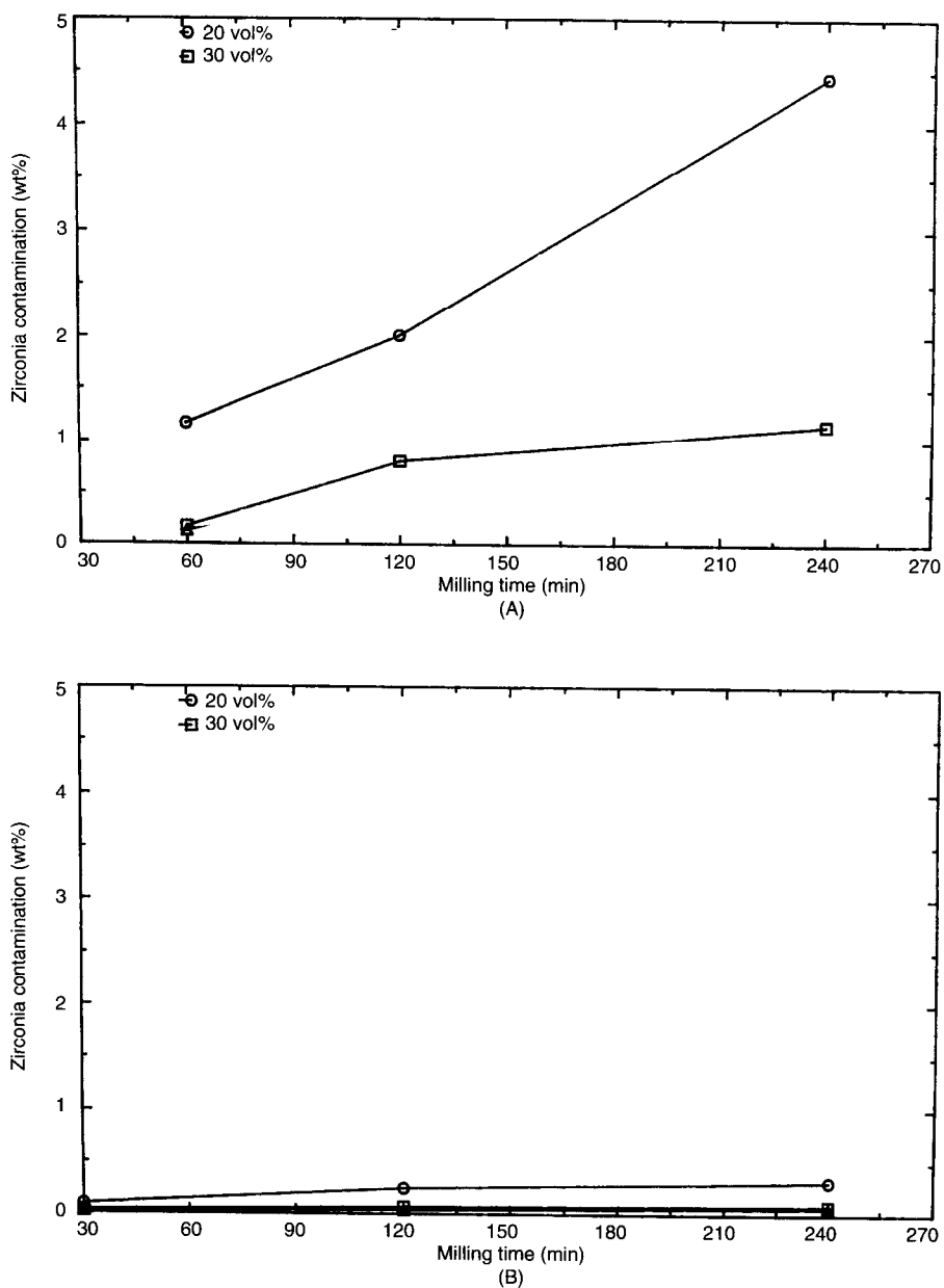
Fig. 8. Variation of media wear product with milling time for different powder loadings in slurry: (A) 6.35-mm media, no deflocculant at 20 and 30 vol % and (B) 1.11-mm media, no deflocculant at 20 and 30 vol %.
