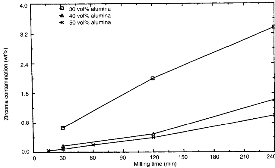
Fig. 3. Dependence of media wear on milling time for different powder loading (4.76-mm media, 900 rpm).
