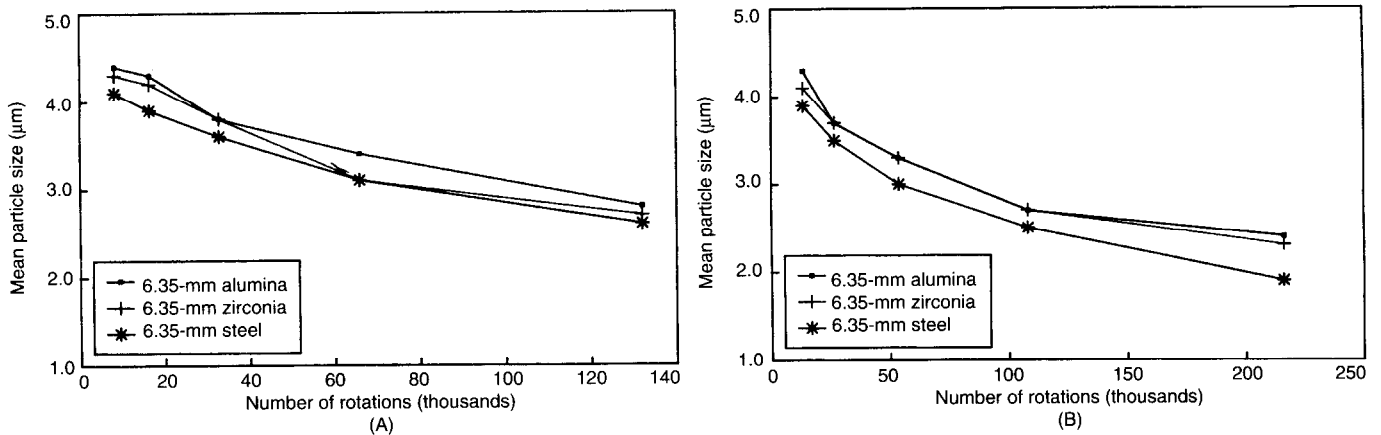
Fig. 4. Dependence of mean particle size on number of mill rotations for different media: (A) 550 and (B) 900 rpm.
