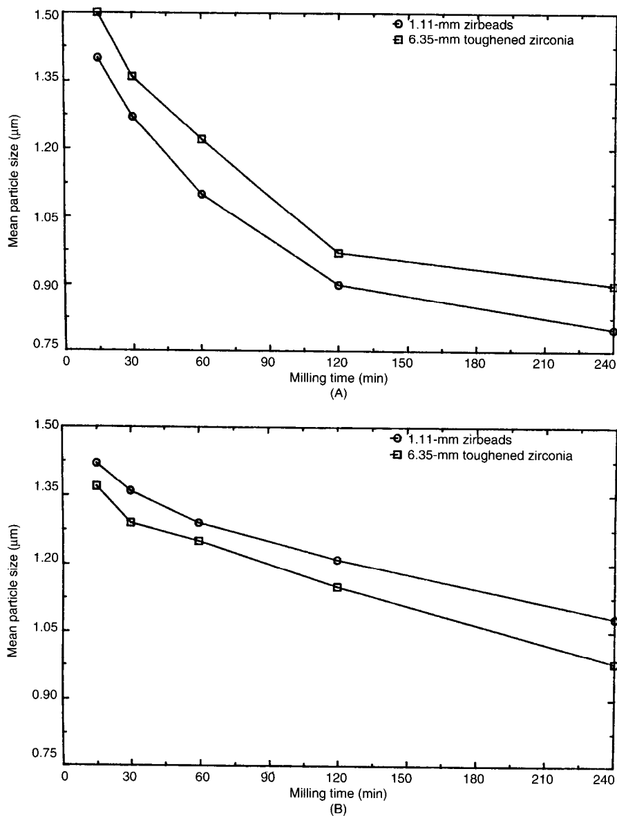
Fig. 6. Dependence of mean particle size of barium titanate powder with time and media size: (A) 30 vol% powder, undeflocculated and (B) 45 vol% powder, deflocculated.
