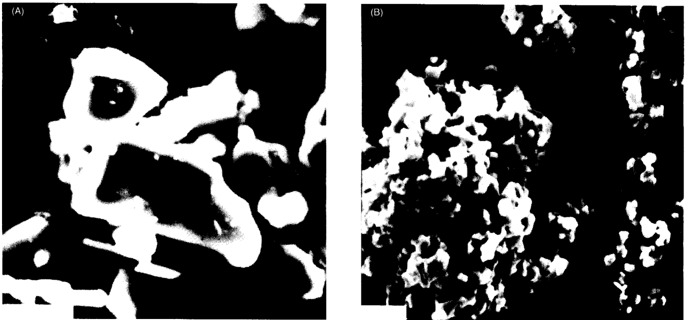
Fig. 7. SEM of as-received powders: (A) alumina and (B) titanate (bar = 2.5 \mu\text{m} ).
